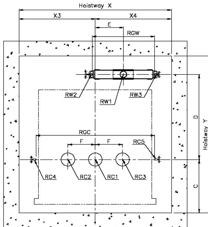
Hoistway Plan
